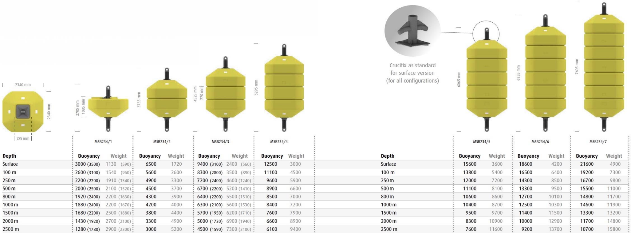
Buoyancy [kgf], weight [kg]. Figures in parentheses are element only - figures in parentheses on configuration MSB234/3 are center element only.
